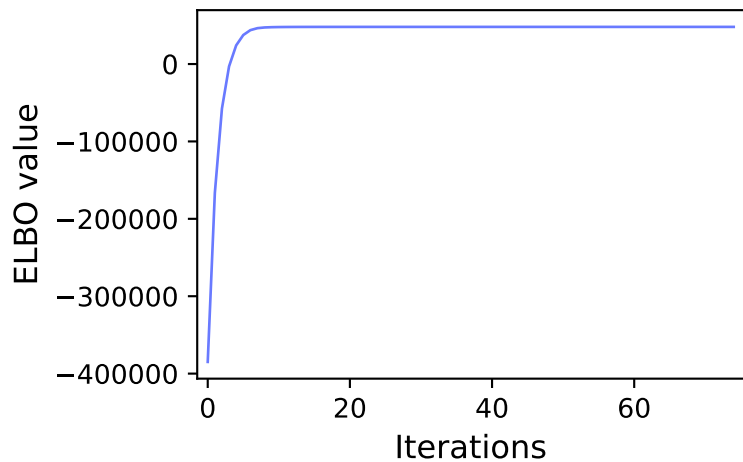
Quantile = 0.75
