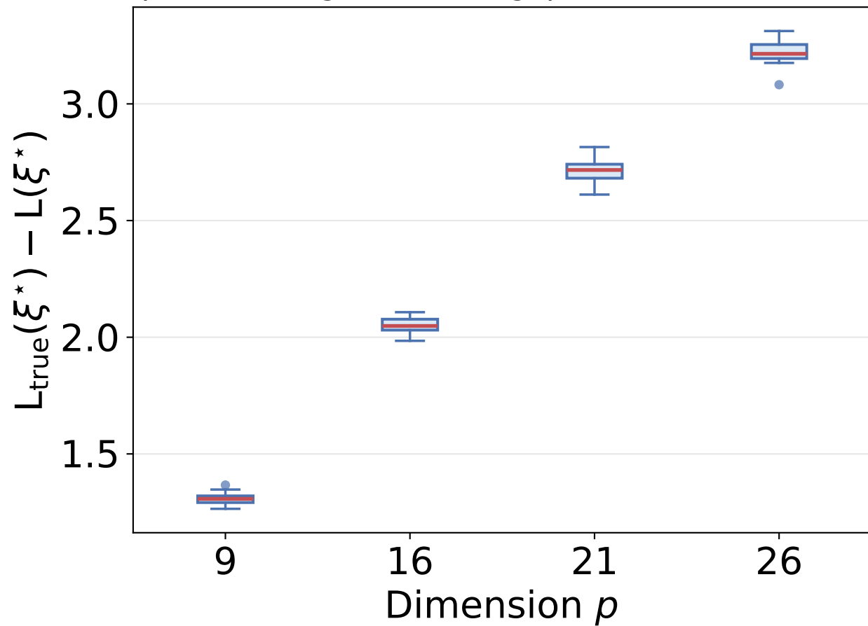
Student's- t Type I SSG post-convergence ELBO gap with fixed n = 1000
