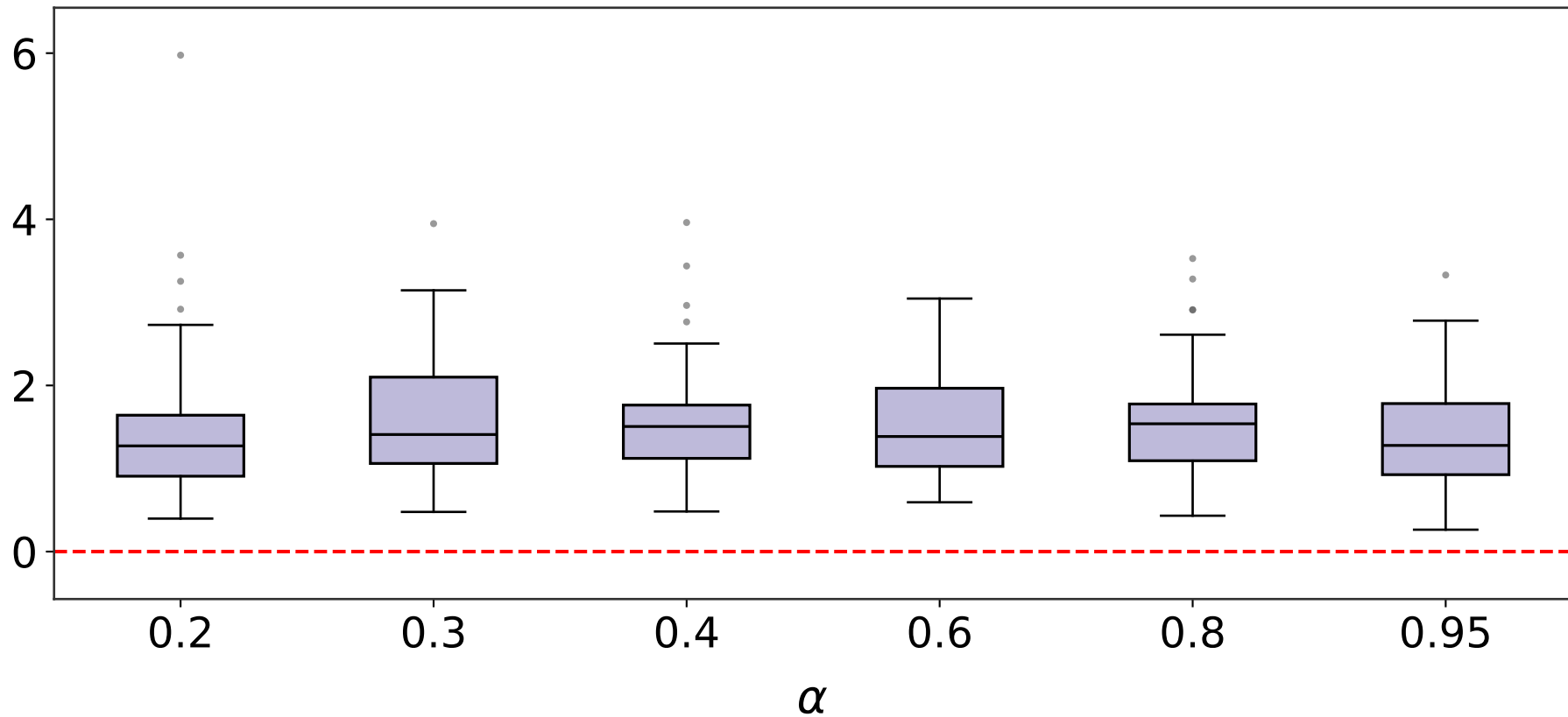
Type I (Laplace) SSG Likelihood
