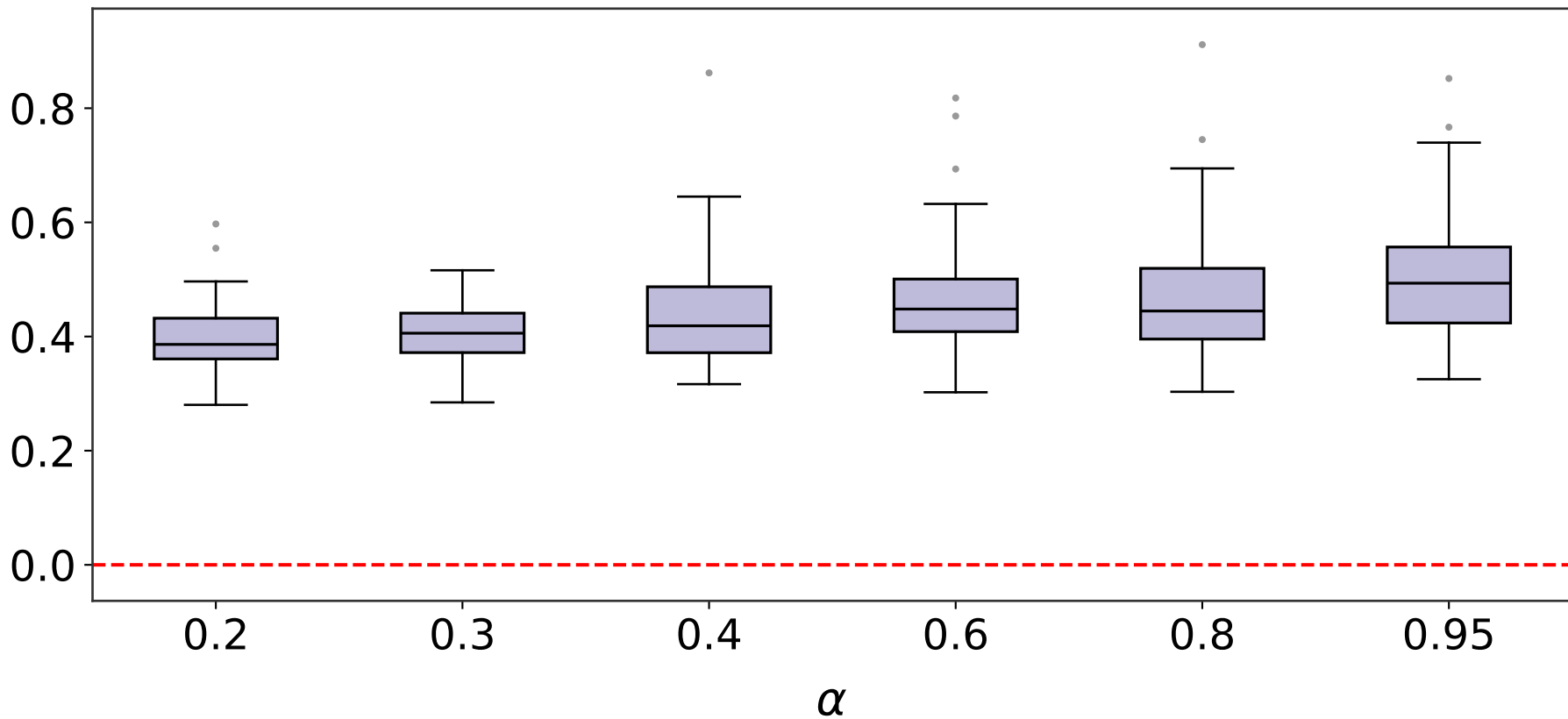
Type II (NB) SSG Likelihood
