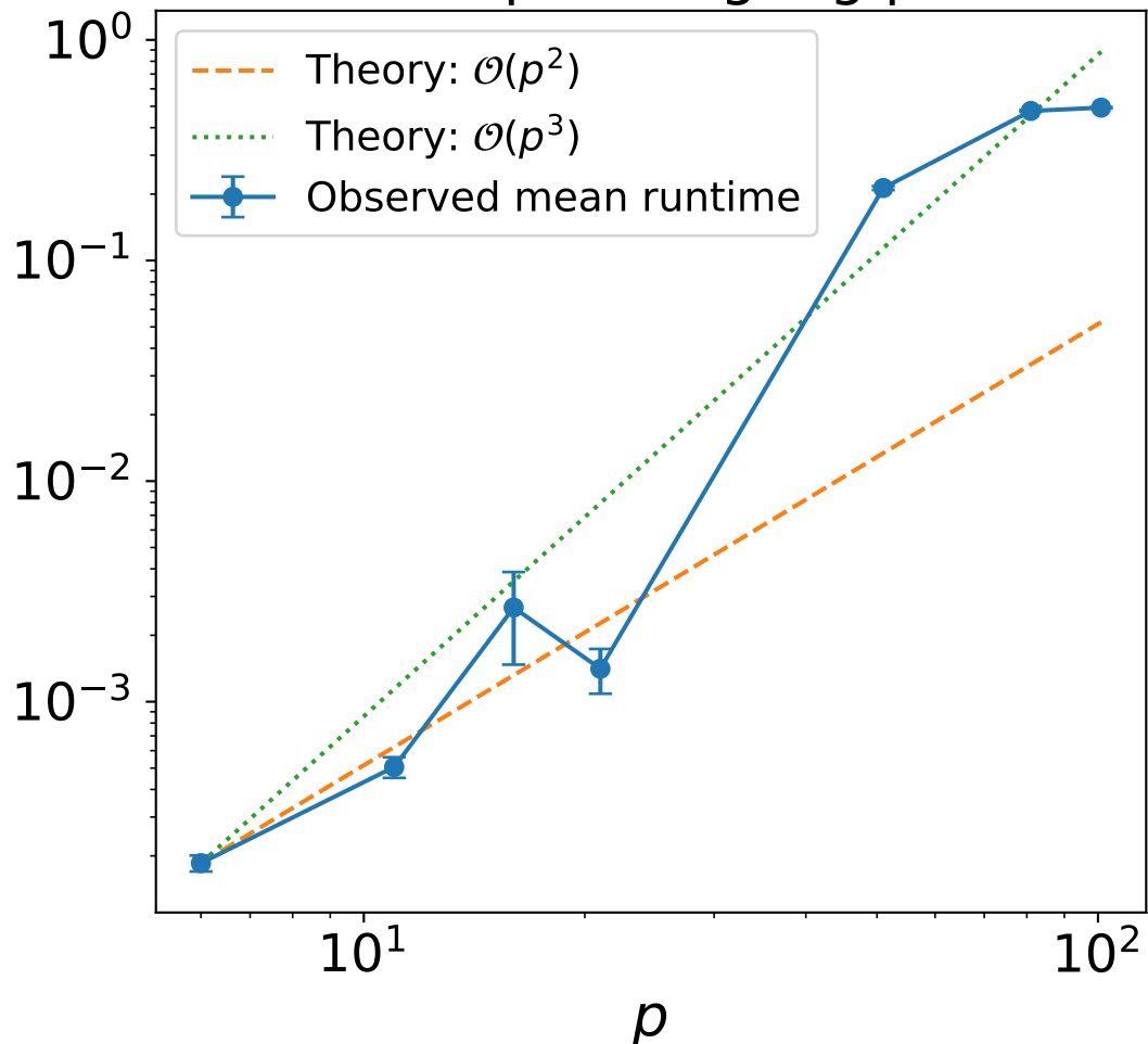
Scaling in p (fixed n = 1000 )
