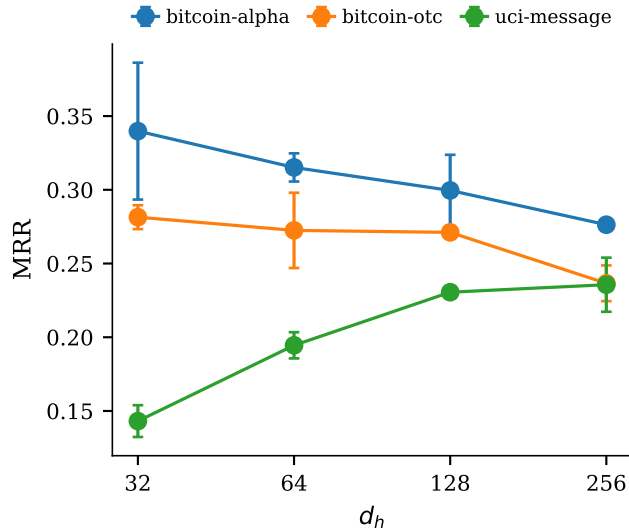
(a) Hidden dimension d_h
