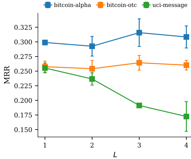
(b) Number of layers L
