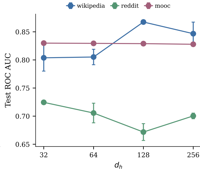
(b) Hidden dimension d_h
