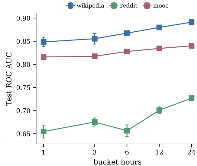
(c) Snapshot width
