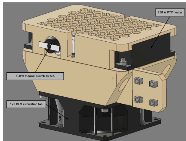
Figure 7 – Chamber-heating assembly showing the 750 W PTC heater, 120 CFM chamber-circulation fan, and independent 150 °C thermal safety switch.
