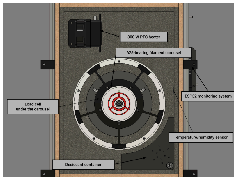
Figure 9 – Integrated filament drybox showing the heated and monitored storage system, desiccant container, load cell, and bearing-supported filament carousel
