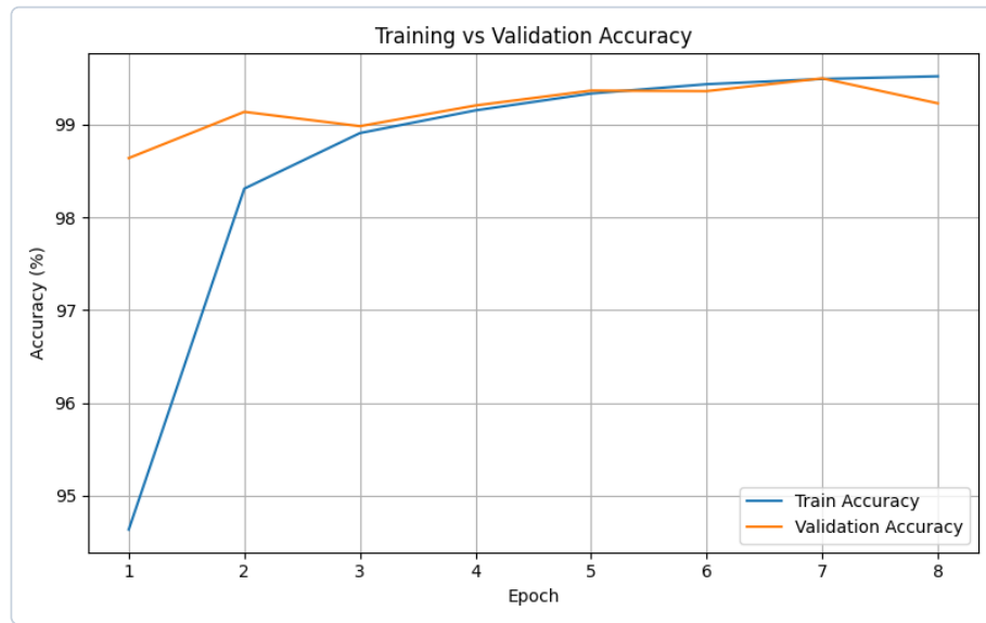
Figure 4. Dataset 2 — Training vs. Validation Accuracy over 8 epochs
