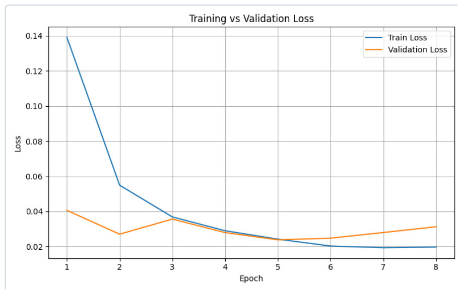
Figure 5. Dataset 2 — Training vs. Validation Loss over 8 epochs
