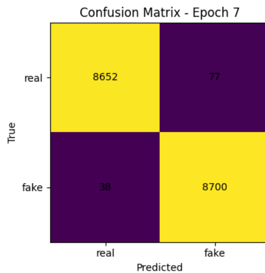
Figure 8: Dataset 2 — Confusion Matrix on the Test Set (Epoch 7). TN = 8,652, FP = 77, FN = 38, TP = 8,700 across 17,467 samples.
