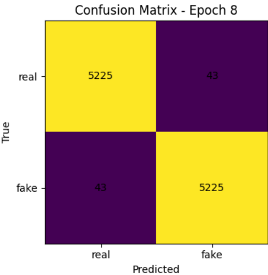
Figure 6: Dataset 1 — Confusion Matrix on the Test Set (Epoch 8). Perfectly symmetric errors: 43 false positives and 43 false negatives out of 10,536 samples.
