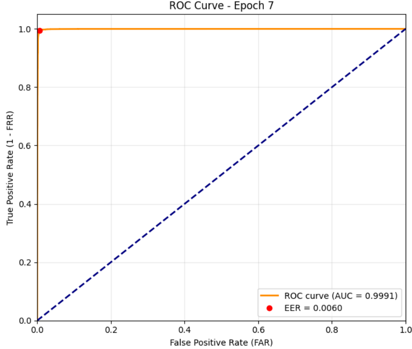
Figure 9: Dataset 2 — ROC Curve (AUC = 0.9991, EER = 0.60%, Epoch 7). Near-perfect discrimination between real and fake samples across all operating thresholds.
