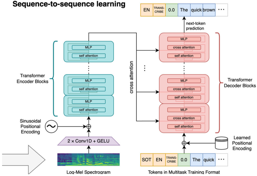
Figure 2: Whisper sequence-to-sequence architecture [16]. The encoder (left) processes a Log-Mel Spectrogram through 2×Conv1D + GELU and stacked Transformer blocks. In FusionGuardNet only the encoder is used; the decoder (right) is discarded after feature extraction.
