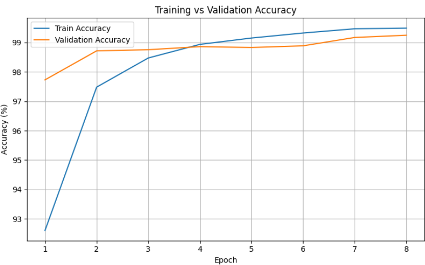
Figure 5: Dataset 1 — Training vs. Validation Accuracy over 8 epochs. The model converges stably, reaching 99.49% training accuracy by epoch 8.
