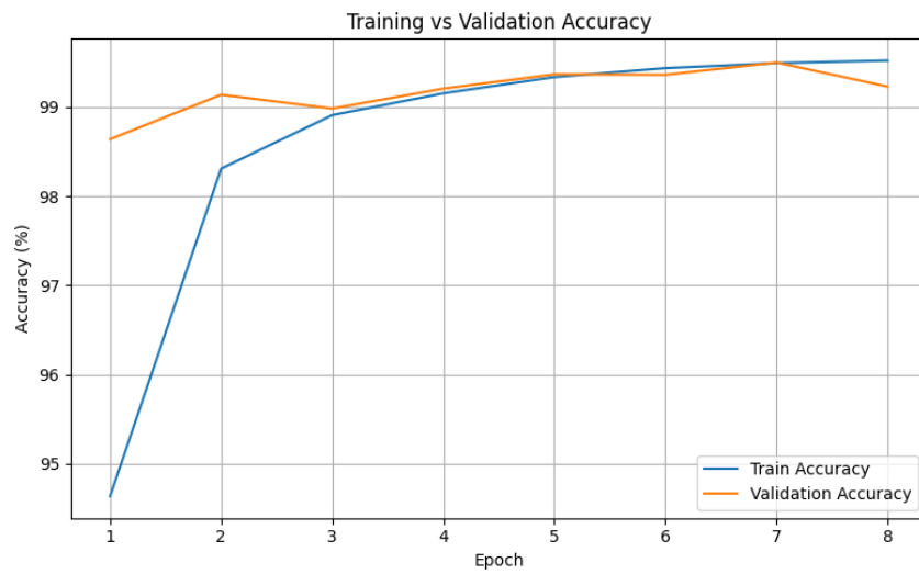
Figure 7: Dataset 2 — Training vs. Validation Accuracy over 8 epochs. The fused model maintains stable convergence on the larger mixed-source dataset.
