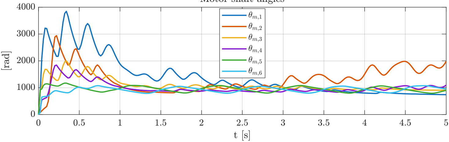
Motor shaft angles
