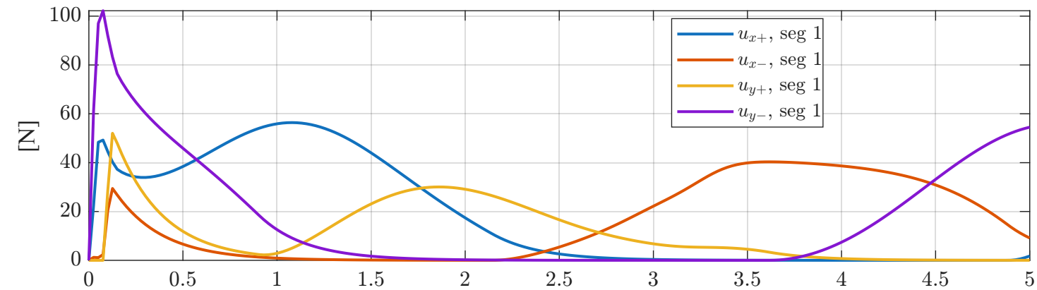
Tendon tensions
