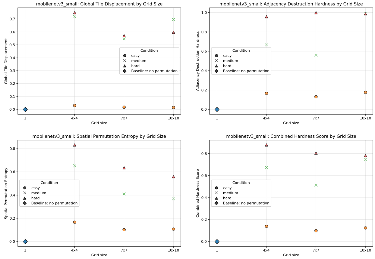
Figure 5: Part 3 hardness metrics by grid size and deterministic difficulty label. The four panels show global tile displacement, adjacency destruction, spatial permutation entropy, and the combined hardness score.
