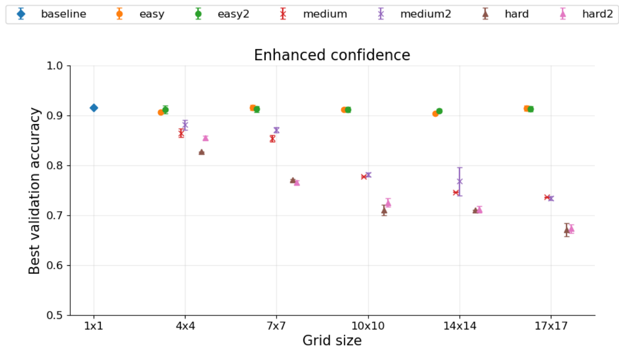
Figure 3: Expanded two-seed Part 1 subset for MobileNetV3-Small. The plot uses seeds 42 and 43, six permutation variants per non-baseline grid, and additional grids through 14 \times 14 and 17 \times 17 . Points show mean best validation accuracy for each permutation variant across completed seeds, with descriptive error bars from the available seed values. The one-tile baseline appears once because it is shared by the expanded run matrix.
