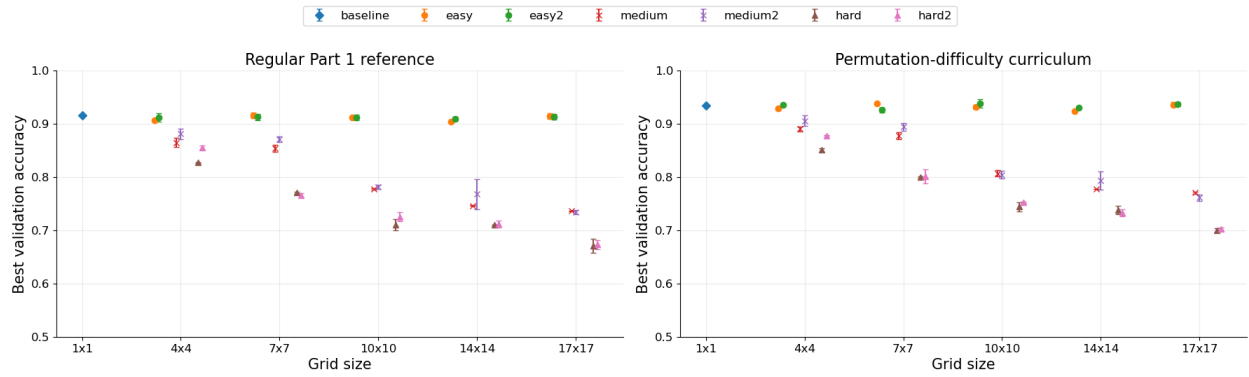
Figure 5: Expanded two-seed Part 2 subset for MobileNetV3-Small. The figure compares the expanded regular Part 1 reference against the expanded permutation-difficulty curriculum using seeds 42 and 43, six permutation variants per non-baseline grid, and additional grids through 14 \times 14 and 17 \times 17 . Points show mean best validation accuracy for each permutation variant across completed seeds, with descriptive error bars from the available seed values.
