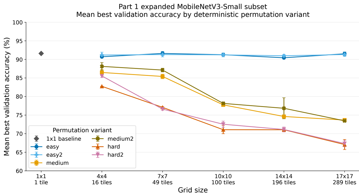
Figure 3: Expanded two-seed Part 1 subset for MobileNetV3-Small. The y-axis reports best validation accuracy in percentage points. Each non-baseline point is one deterministic permutation variant at one grid size, averaged across seeds 42 and 43; error bars show the descriptive standard deviation across those two seed values, not standard error or confidence intervals. The non-baseline coverage is complete for five grids ( 4 \times 4 , 7 \times 7 , 10 \times 10 , 14 \times 14 , and 17 \times 17 ), six variants per grid, and two seeds. The six non-baseline variants are easy , easy2 , medium , medium2 , hard , and hard2 . The one-tile baseline appears once because it is shared by the expanded run matrix and has a single saved seed-42 run rather than a separate seed-43 rerun. These results are descriptive and do not imply statistical significance.
