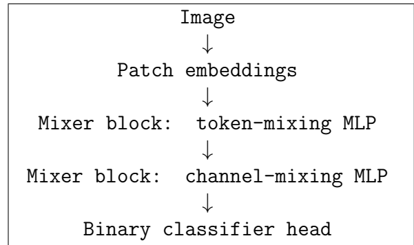
Figure 2: Simplified MLP-Mixer flow. Token mixing exchanges information across patches, while channel mixing recombines features within each patch representation.
