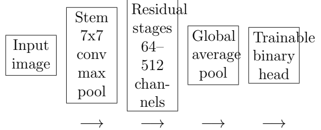
Figure 1: Schematic overview of the ResNet-18 flow used in the experiments. The ImageNet-pretrained residual backbone is frozen; only the final binary head is optimized, except that the Part 2 MLP-head ablation replaces the linear head with a small nonlinear head.
