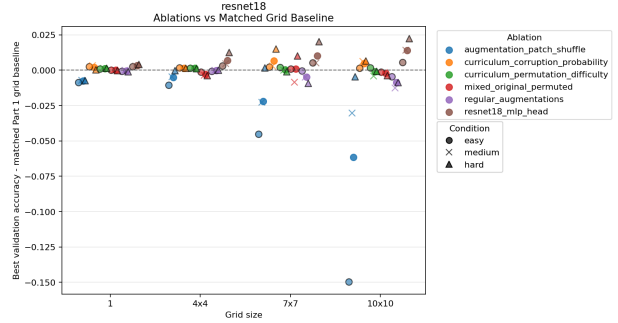
Figure 3: Part 2 best-validation-accuracy delta from the matched ResNet-18 baseline. Positive values indicate improvement relative to the same grid size and deterministic permutation preset.
