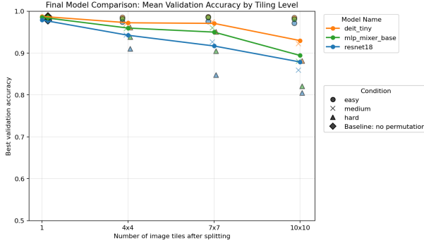
Figure 2: Part 1 mean best validation accuracy as a function of tile count for the three frozen pretrained backbones. Higher tile counts correspond to finer grids and more opportunities for tile-wise spatial disruption.
