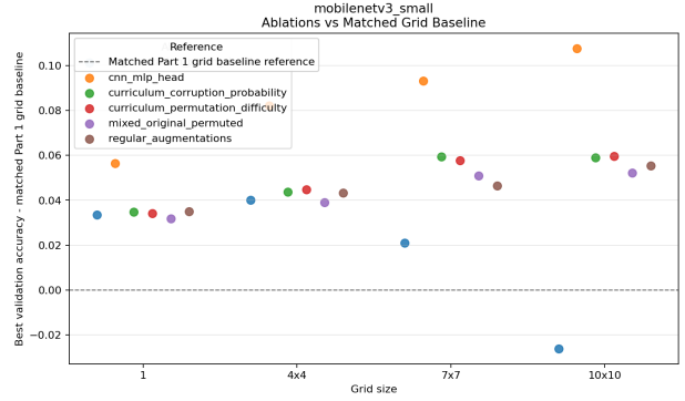
Figure 5: Part 2 best-validation-accuracy delta from the matched CNN baseline. Positive values indicate improvement relative to the same grid size and deterministic permutation preset; negative values indicate that the ablation underperformed the matched baseline.
