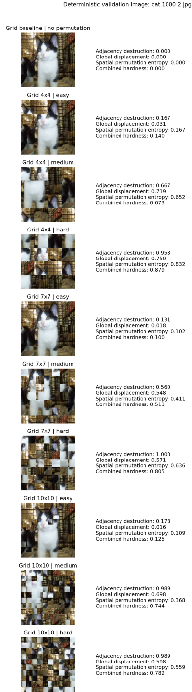
Figure 6: Part 3 example permutations and model-agnostic hardness metrics for the deterministic grid and difficulty settings. The figure is intended to make the easy, medium, and hard presets visually comparable across grid sizes.
