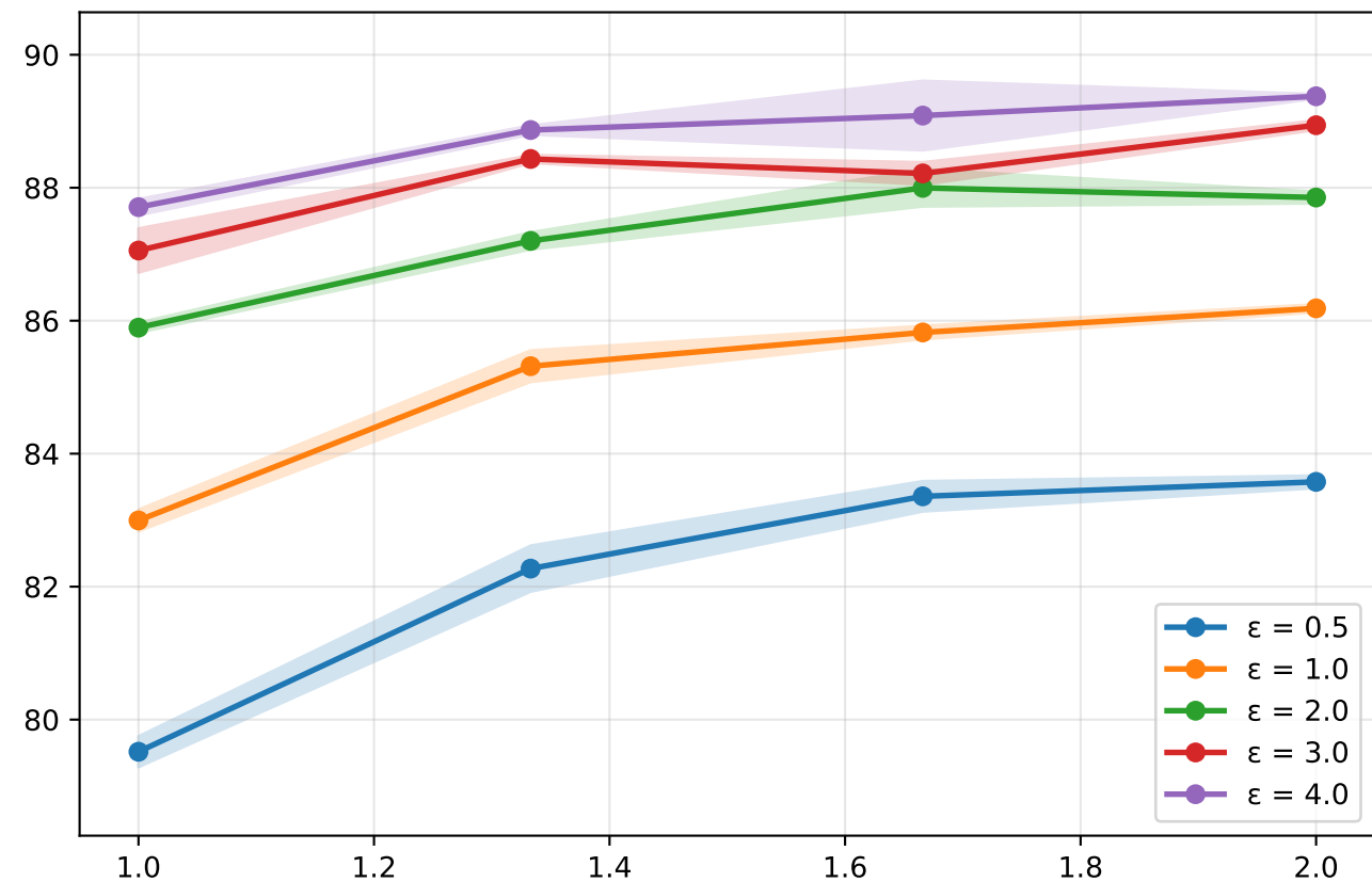
FCN on Adult
