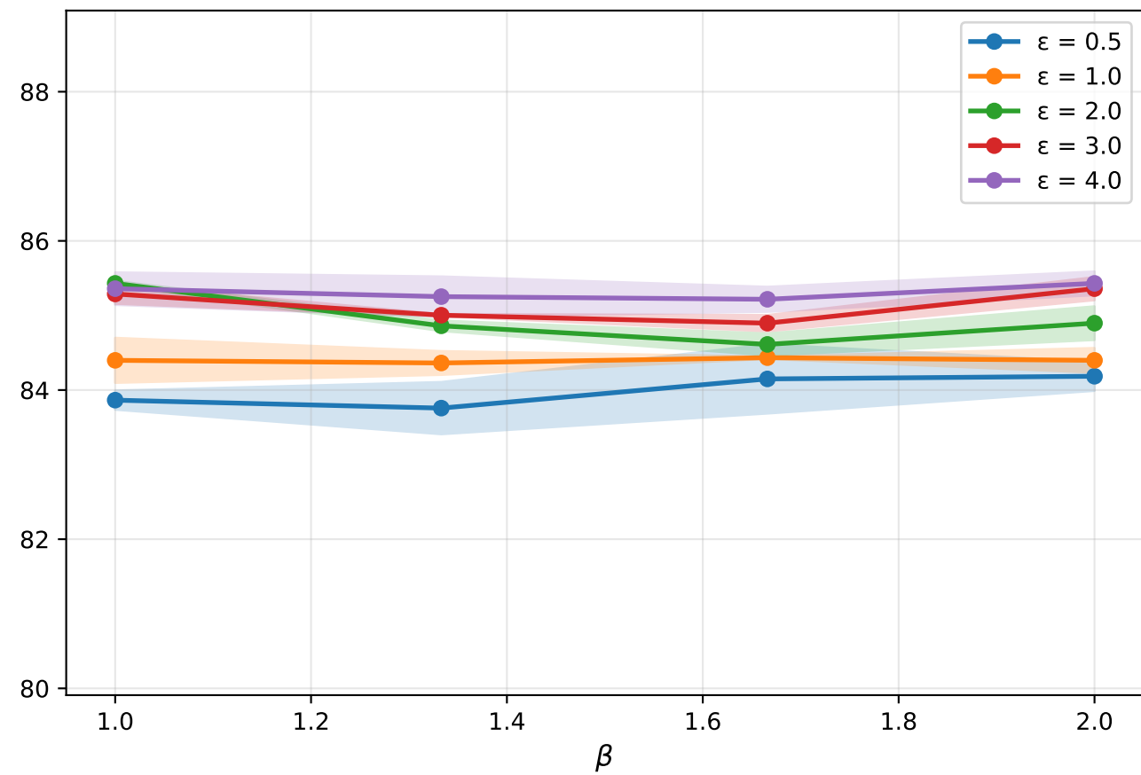
FCN on Adult
