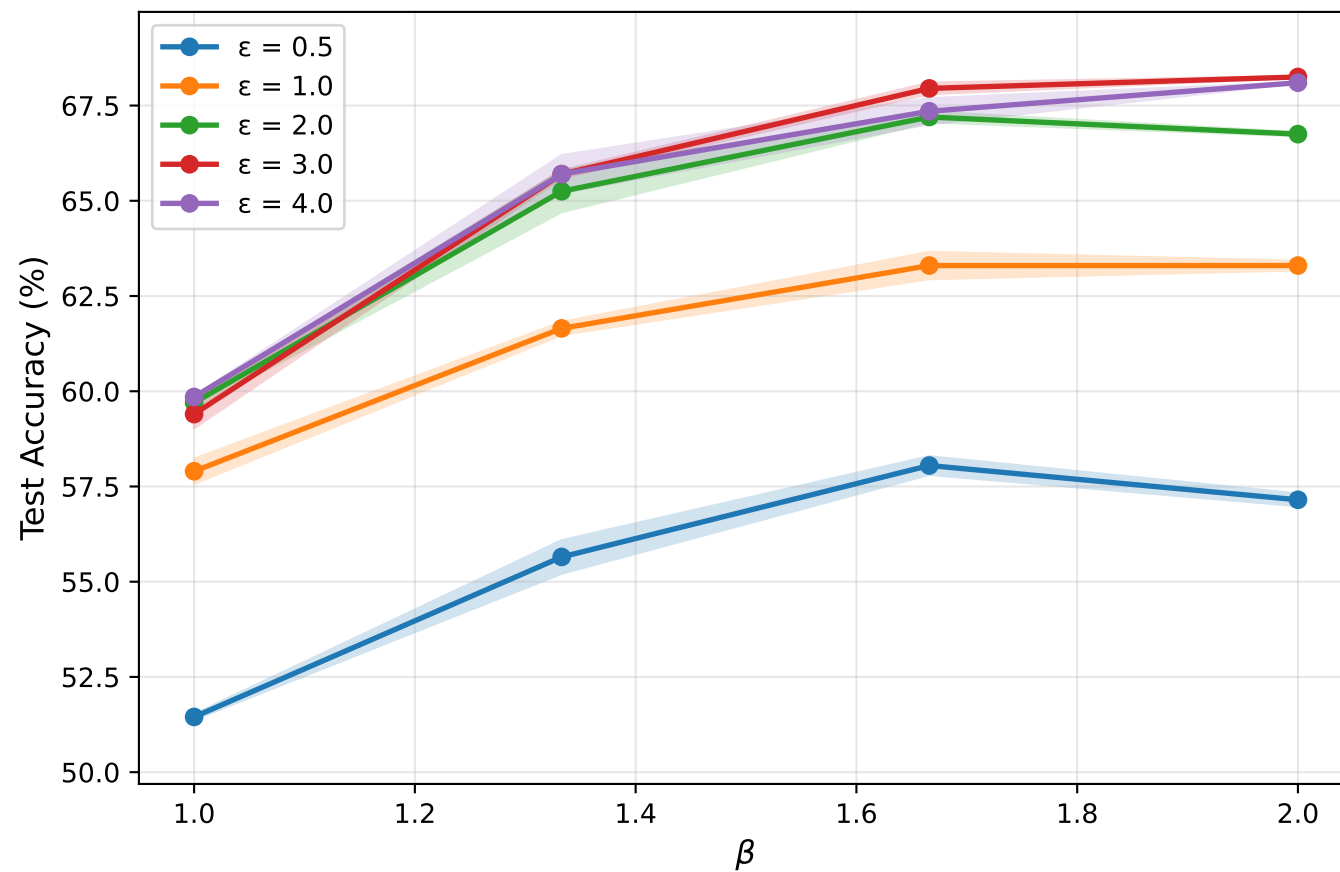
ScatterNet on CIFAR-10
