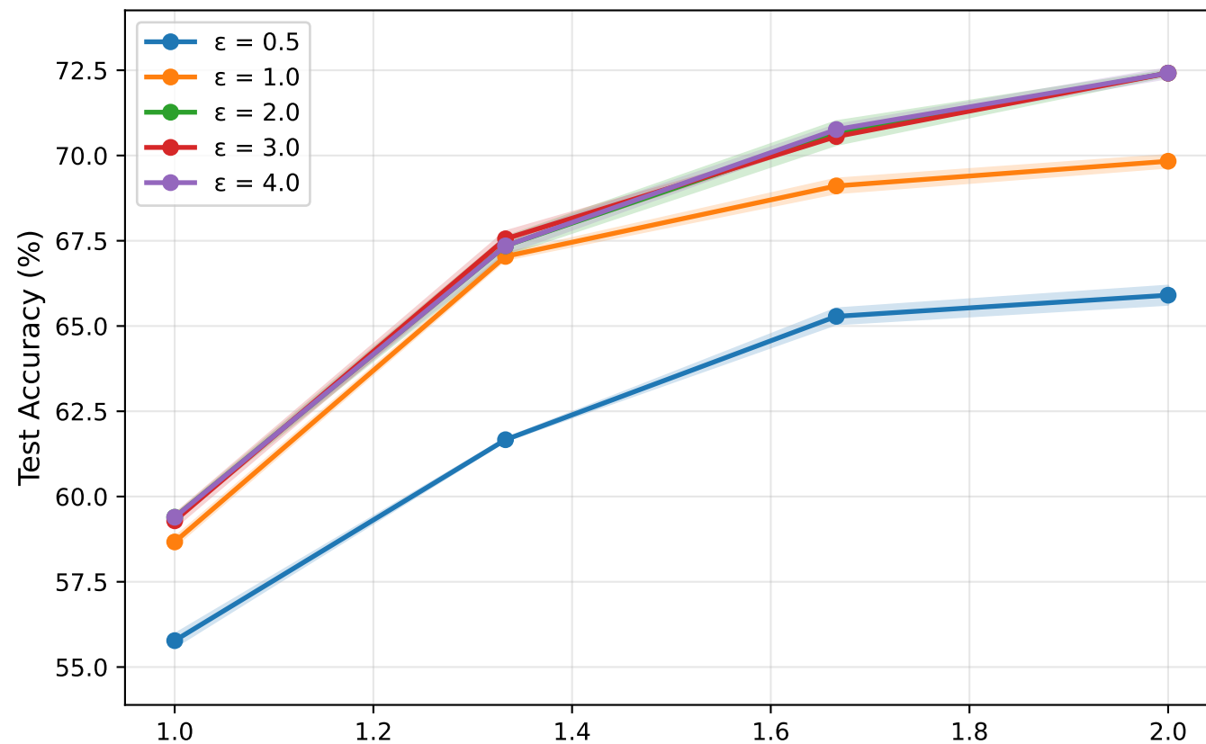
ScatterNet on CIFAR-10
