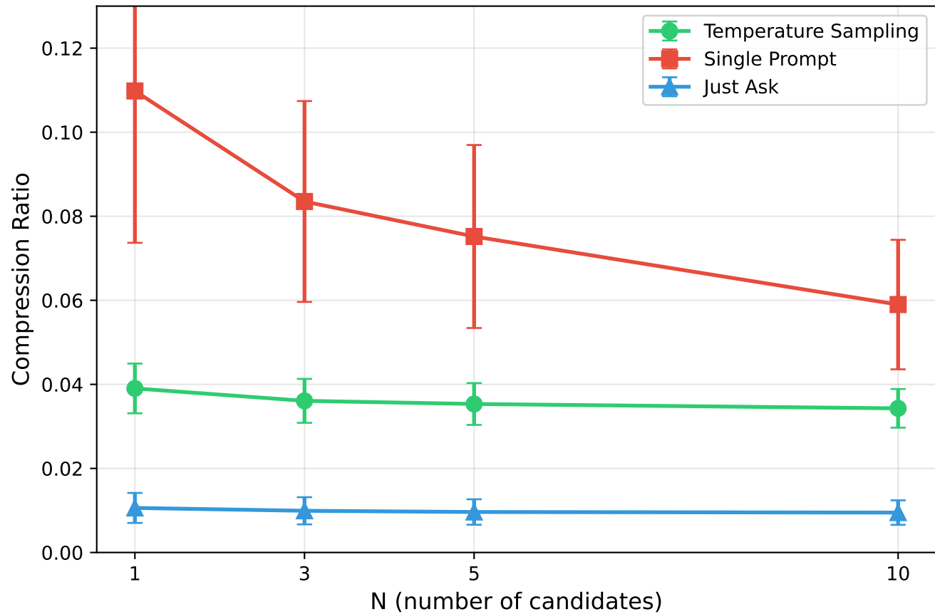
MBPP
