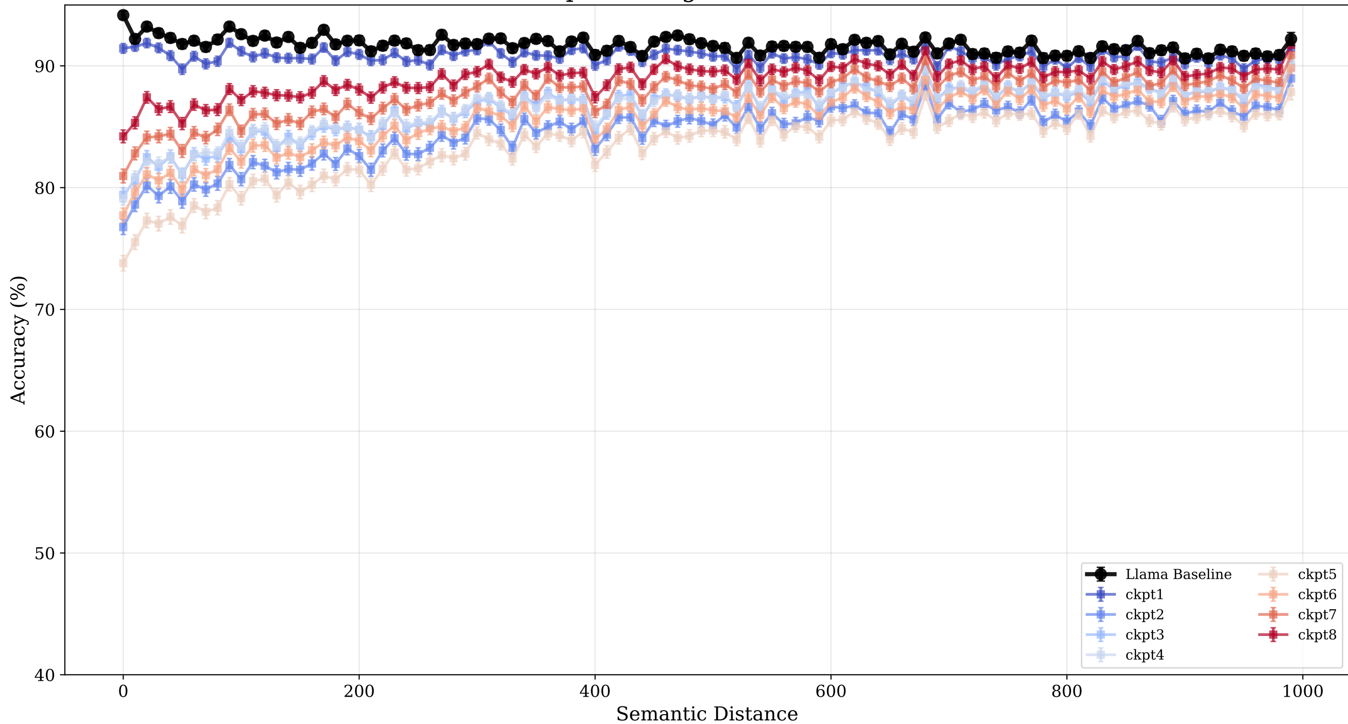
Checkpoint Progression: Llama-RR
