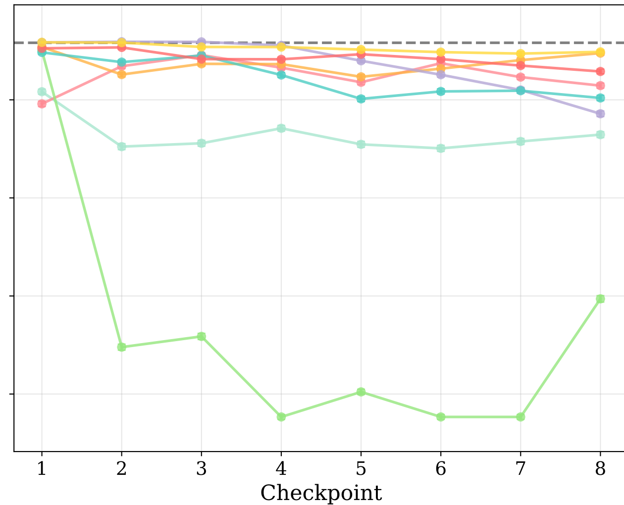
Distance = 500
