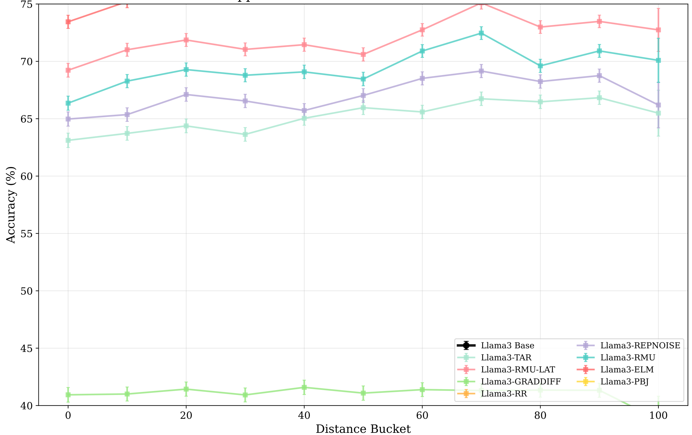
Ripple Effects: Base vs Unlearned Models
