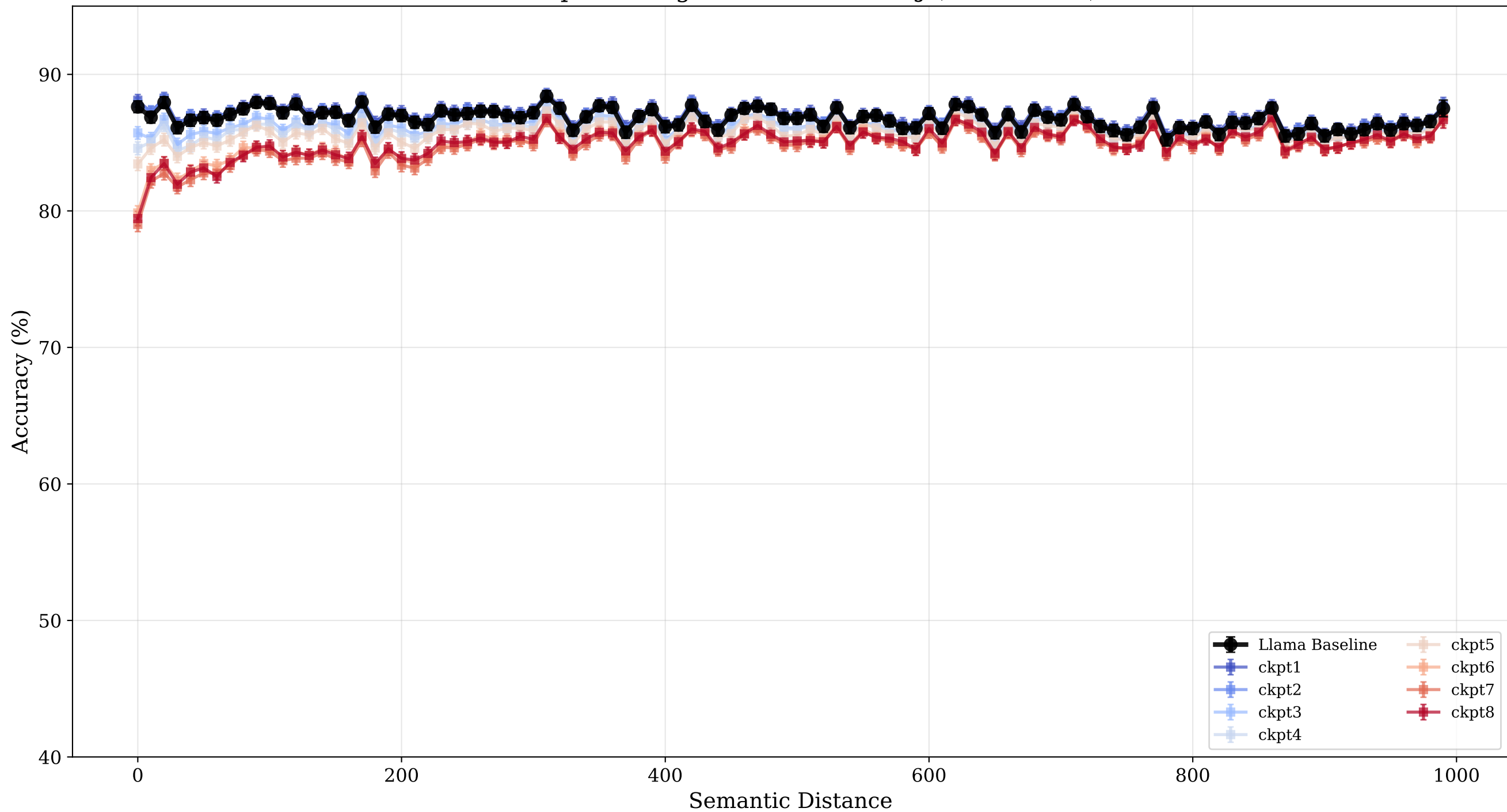
Checkpoint Progression: Llama-PBJ (Fixed Scale)
