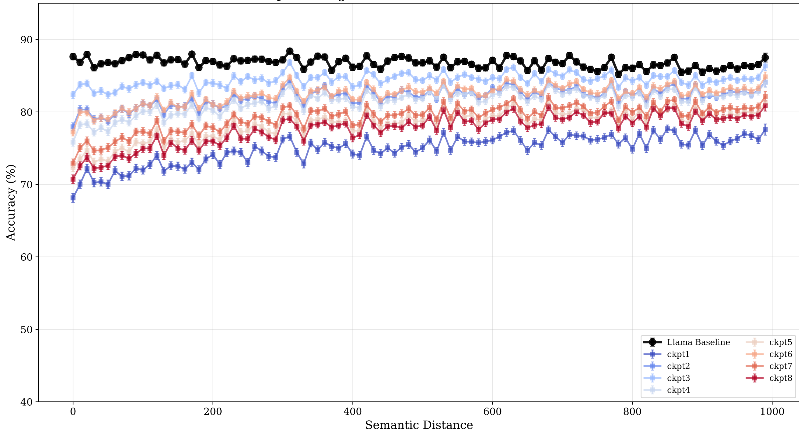
Checkpoint Progression: Llama-RMU-LAT (Fixed Scale)
