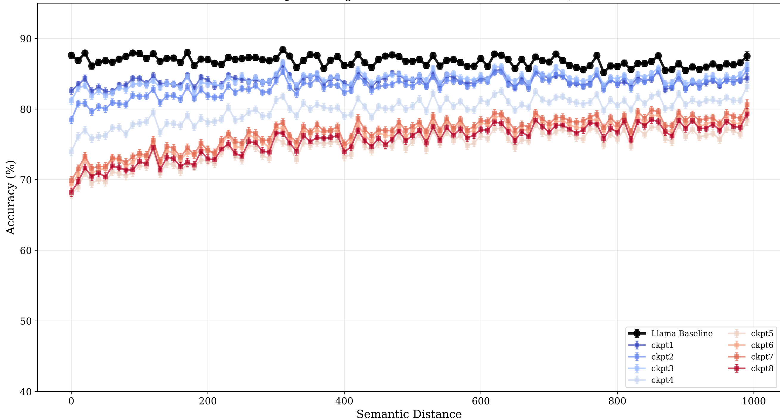
Checkpoint Progression: Llama-RMU (Fixed Scale)
