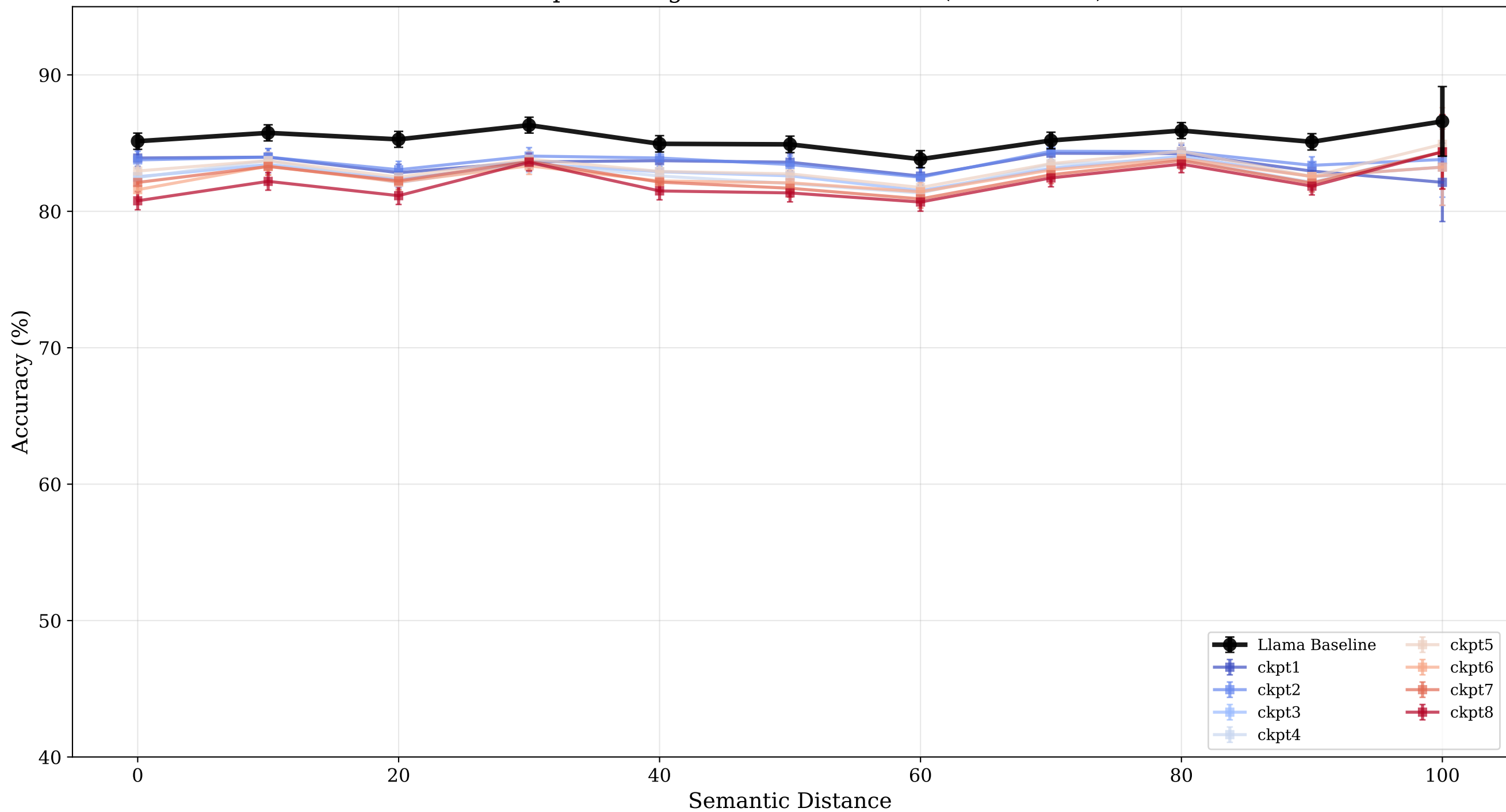
Checkpoint Progression: Llama-ELM (Fixed Scale)
