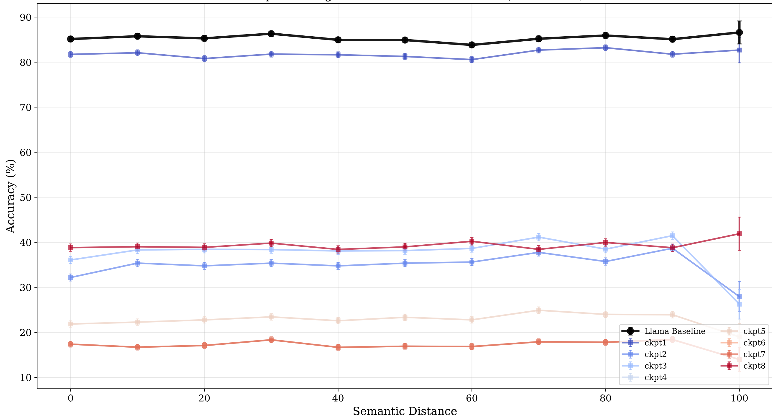
Checkpoint Progression: Llama-GRADDIFF (Auto Scale)
