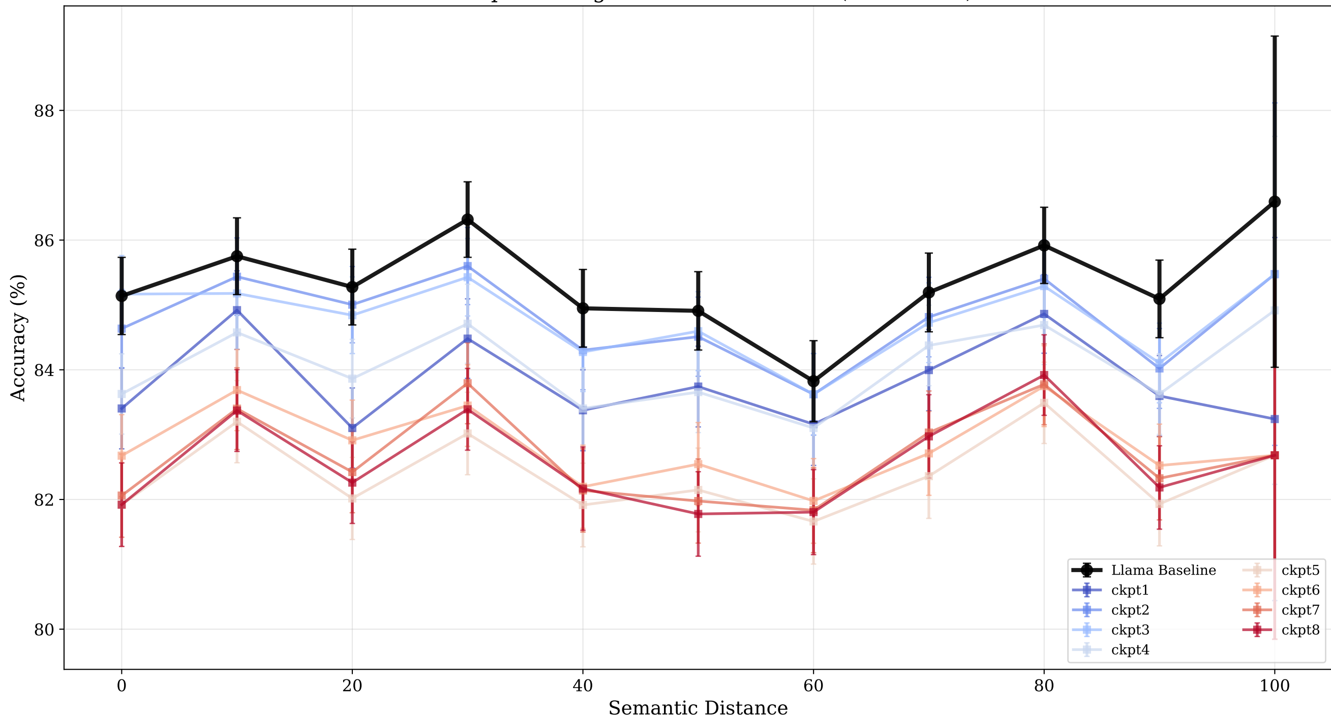
Checkpoint Progression: Llama-RMU (Auto Scale)
