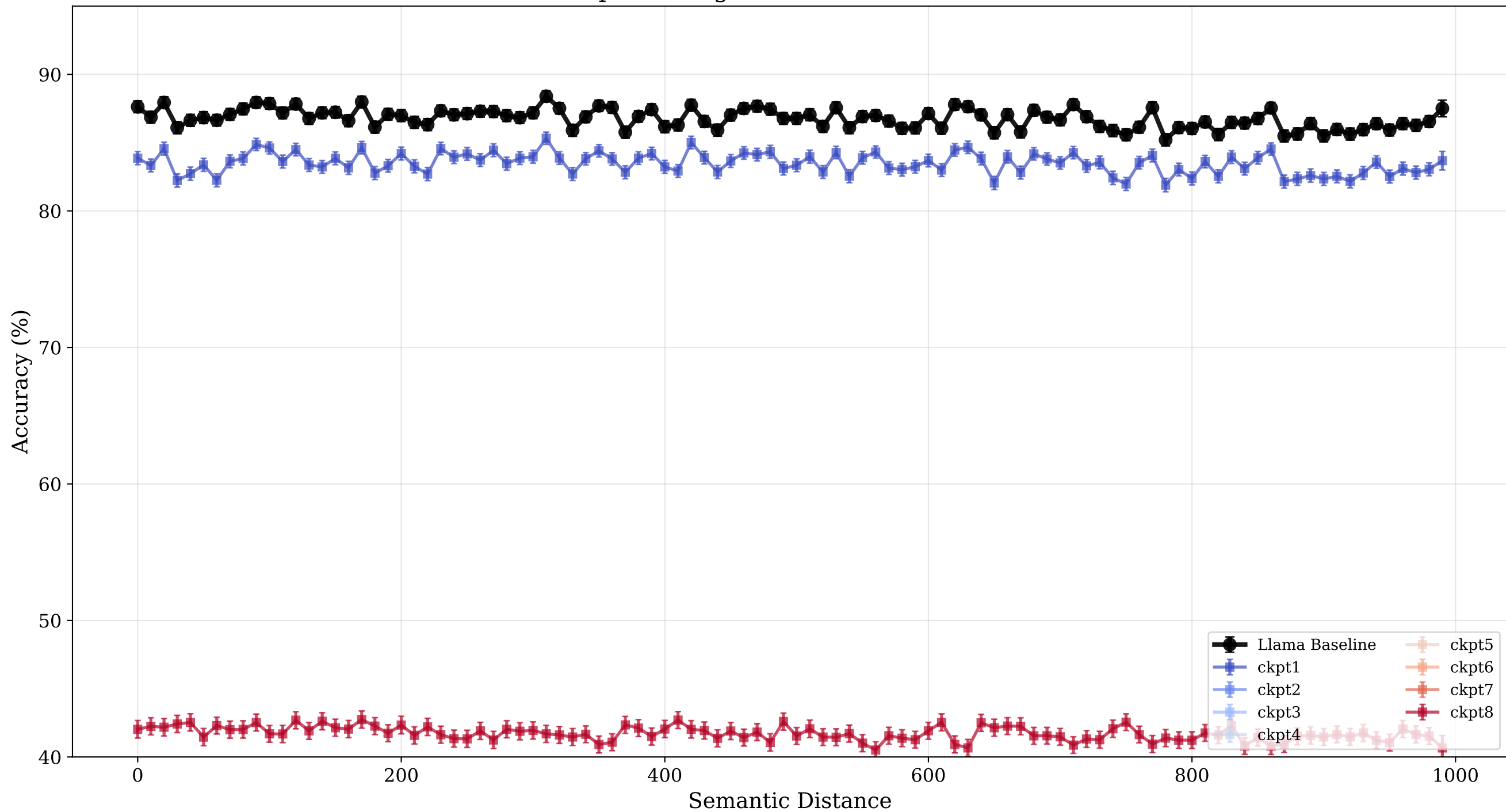
Checkpoint Progression: Llama-GRADDIFF
