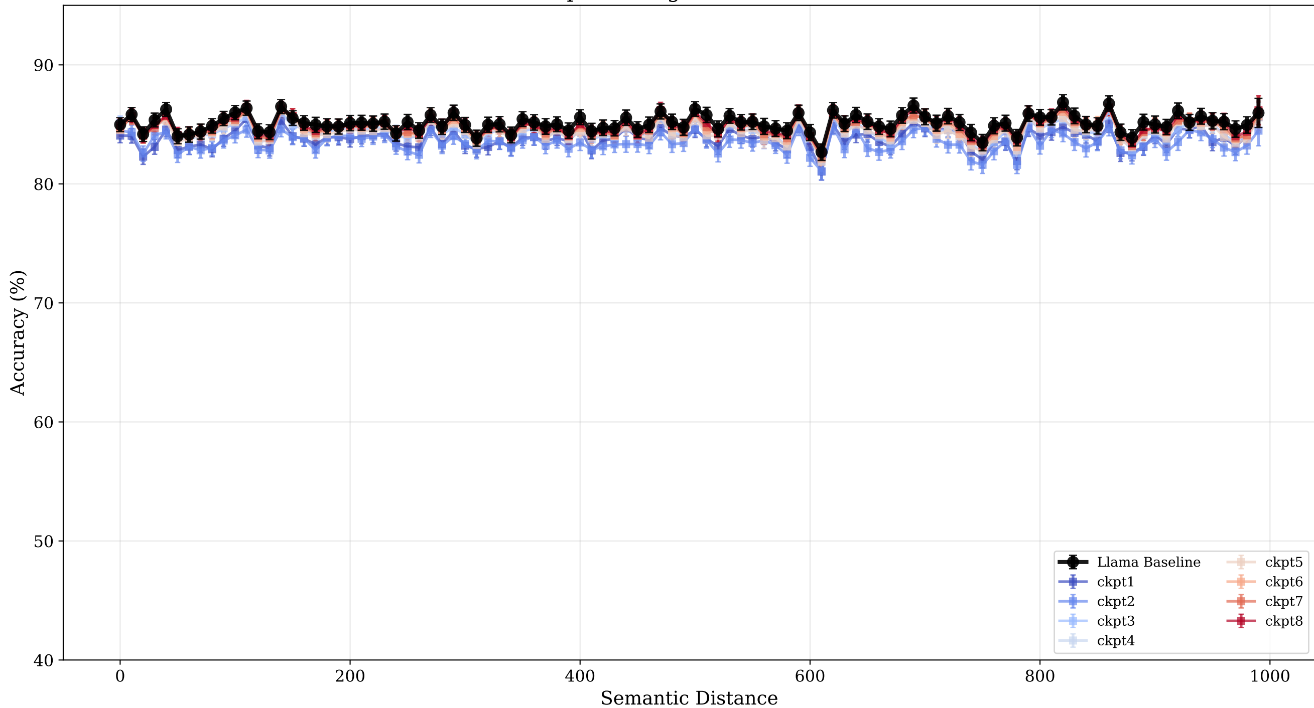
Checkpoint Progression: Llama-RR
