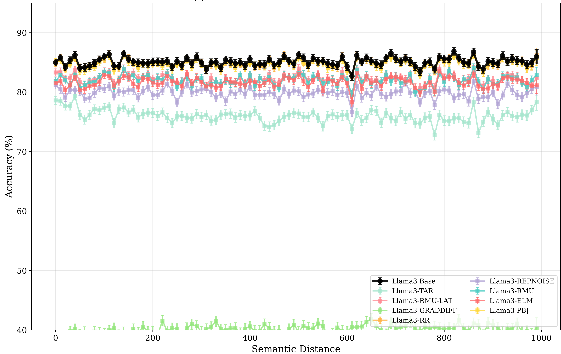
Ripple Effects: Base vs Unlearned Models
