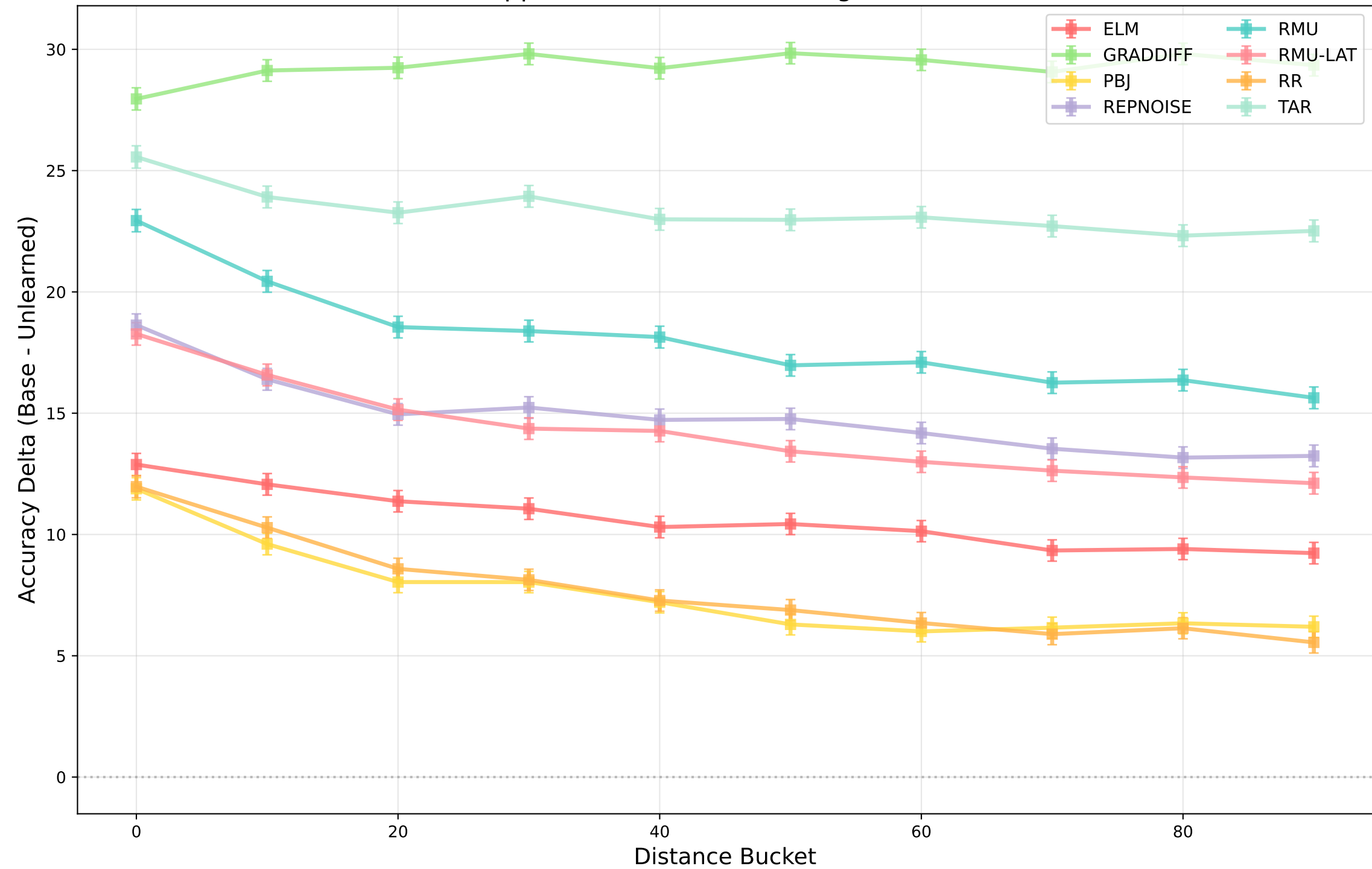
Ripple Effects: All Unlearning Methods
