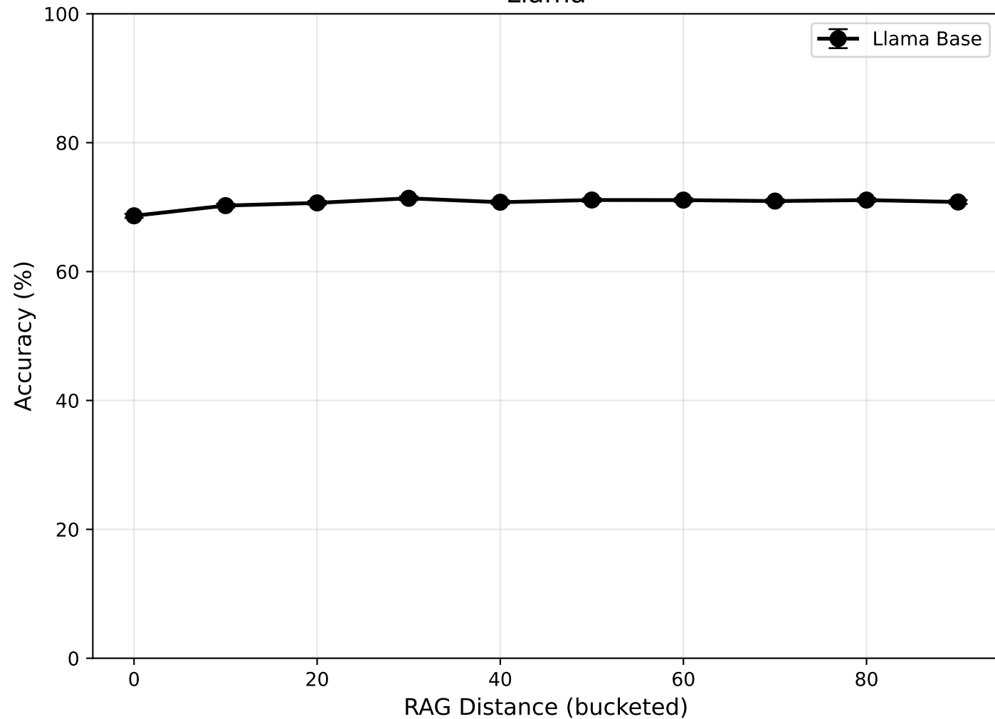
Base Model Accuracy vs RAG Distance Llama
