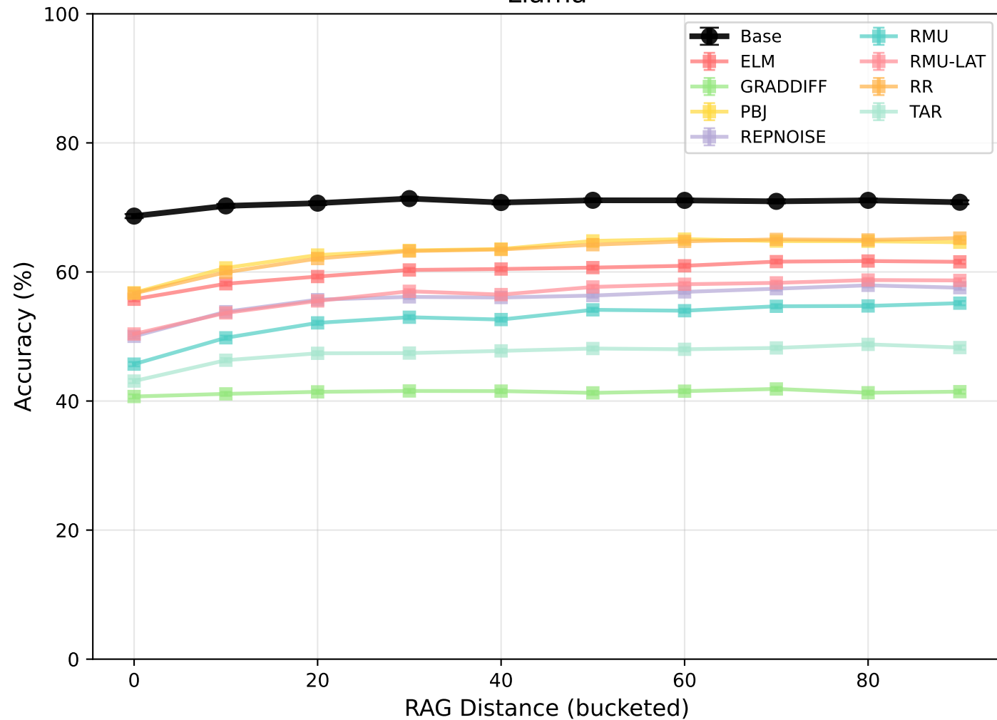
RAG Distance vs Accuracy: All Methods Llama
