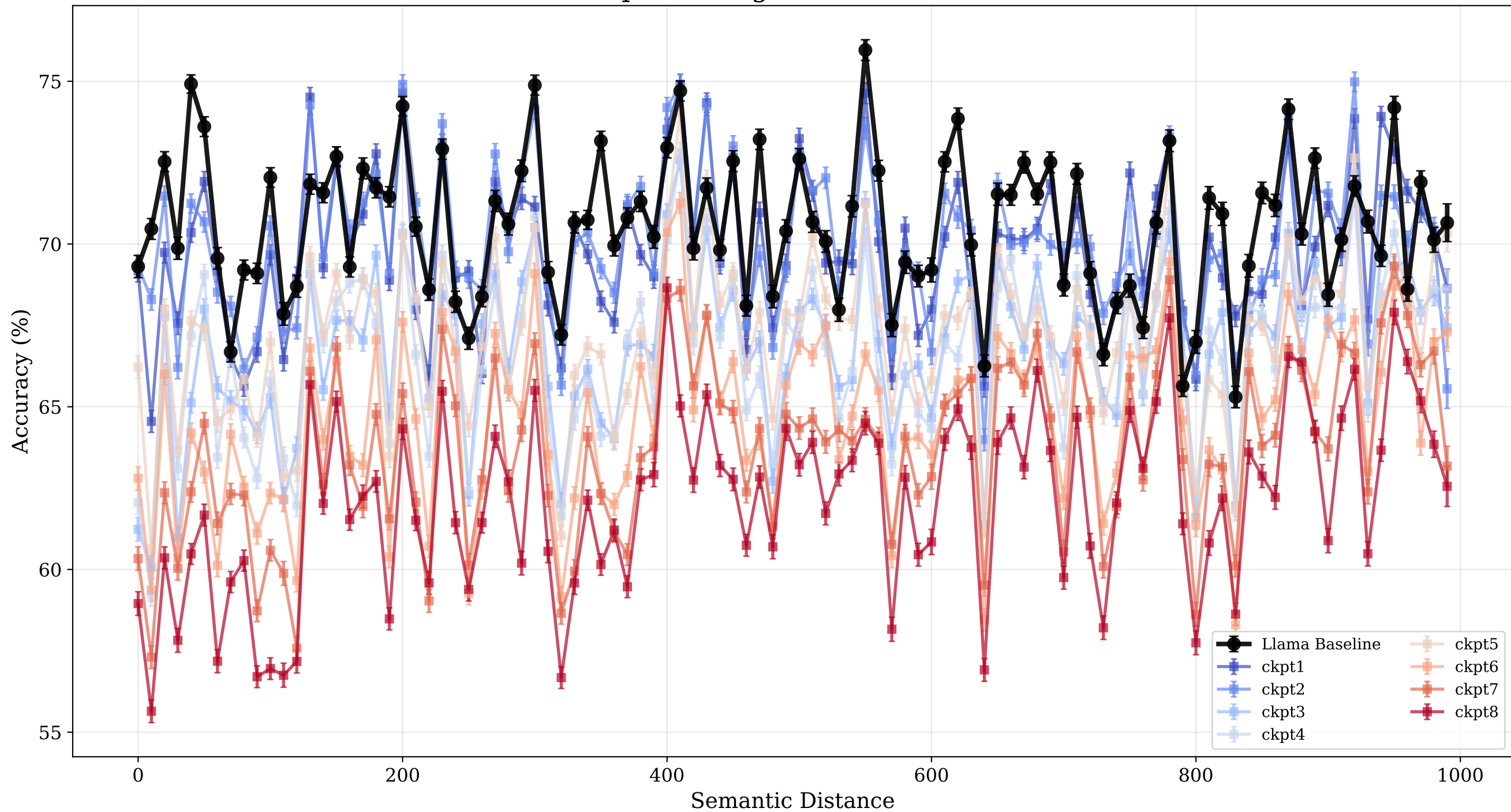
Checkpoint Progression: Llama-ELM
