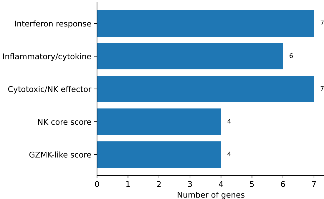
Fig. S3. Curated module sizes
