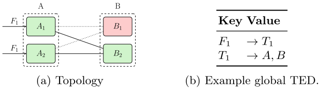
Fig. 1. A sample topology and corresponding TED. (Color figure online)
