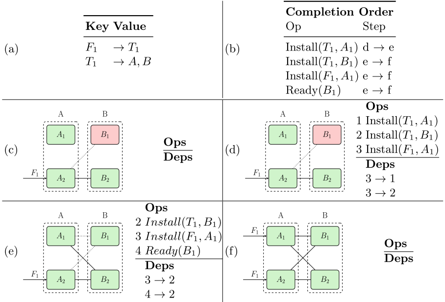
Fig. 2. This shows a sample run of our model with one domain recovering and a total of four ops. Part (a) shows the desired TED. Part (b) shows the order the ops are completed, and the steps between which they finish. Parts (c)–(f) show snapshots of the state at different points in the model run.
