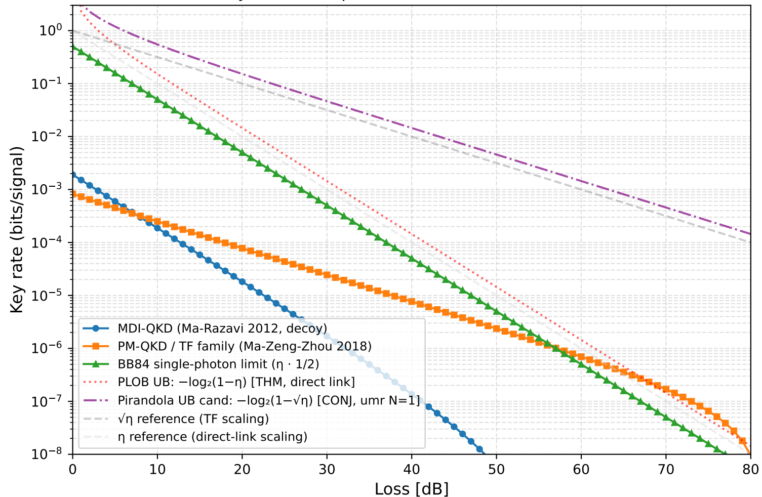
DV-QKD Family Pareto Map: BB84 / MDI / PM-QKD vs UB candidates
