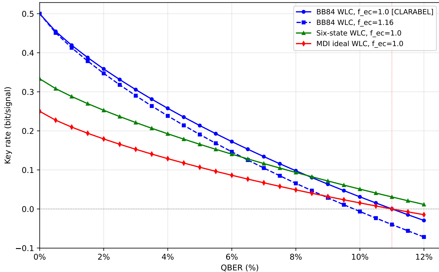
Phase 0 Integration: BB84 / Six-state / MDI via WLC SDP (Winick-Lütkenhaus-Coles 2018 Fig.3 reproduction)
