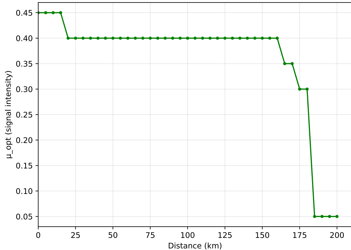
Optimal signal intensity vs distance
