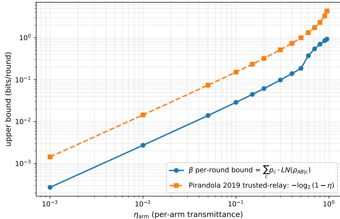
\beta path vs Pirandola (qubit amp-damp post-BSM)
