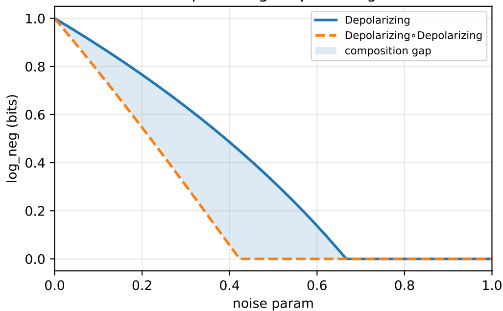
Depolarizing \circ Depolarizing
