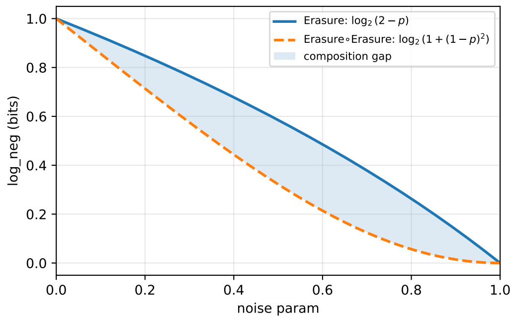
Erasure \circ Erasure
