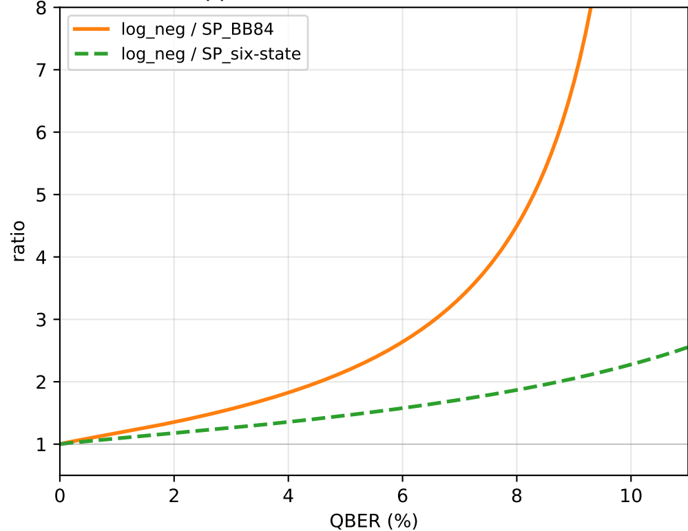
PPT-relaxed upper bound looseness vs achievable SP rate
