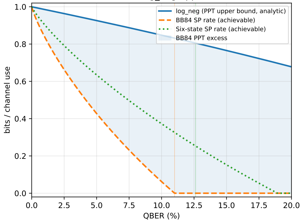
MS-EB BB84/six-state: log_neg upper vs SP achievable
