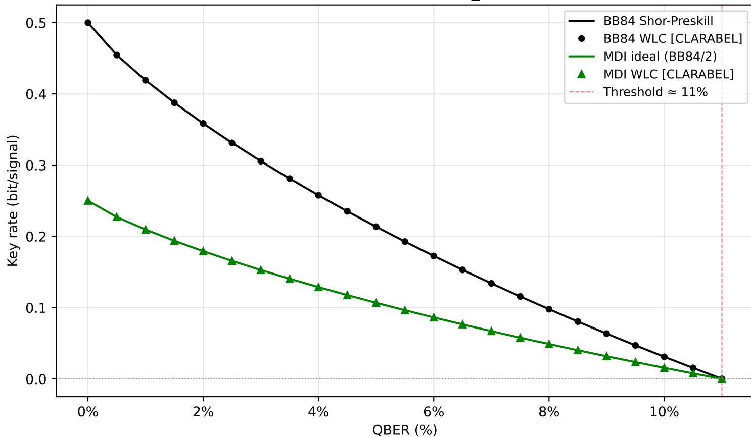
BB84 vs ideal MDI-QKD ( f_{ec}=1.0 )
