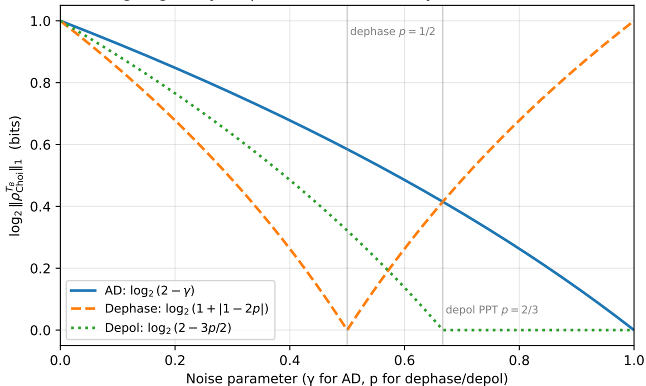
Log-negativity of qubit Choi states (analytic formulas, [SYN])
