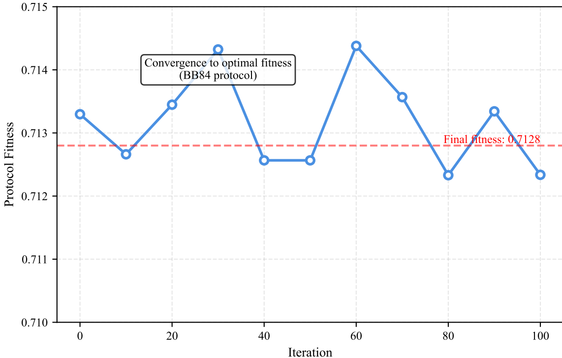
Evolution of Protocol Fitness over 100 Iterations
