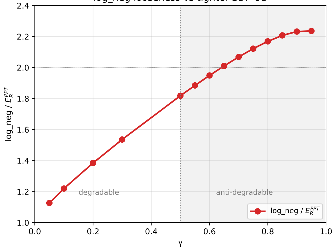
\log\_neg looseness vs tighter SDP UB
