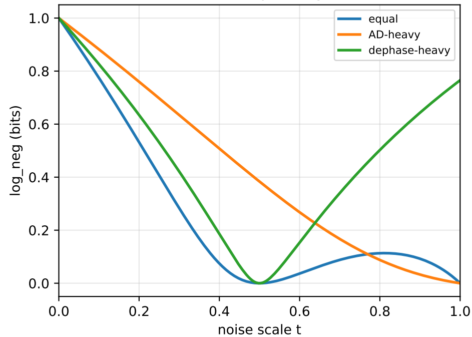
AD \circ Dephasing
